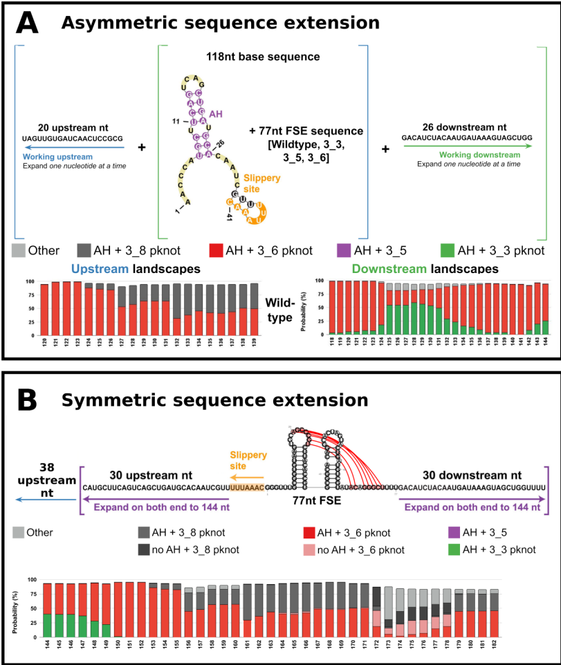
Figure 2. Conformational landscapes of the wild-type FSE with upstream or downstream extensions of sequence (top) and symmetric extensions of sequence (bottom). (A) In the conformational landscapes with increasing upstream or downstream sequence, the ensemble of 2D folds at each sequence length is predicted by NUPACK. 38 For each length, probabilities of 2D folds are calculated from the Boltzmann factor, and all structures containing AH and 3_6, 3_3, or 3_5 motifs are individually summed. Motifs containing 3_6 and AH are in red; motifs containing 3_3 and AH are in green; and motifs containing 3_5 and AH are in purple. See Figure 4 for examples of folds at different lengths. (B) The bottom landscape is computed with a symmetric extension on both ends of the 144-nt segment containing the FSE.
